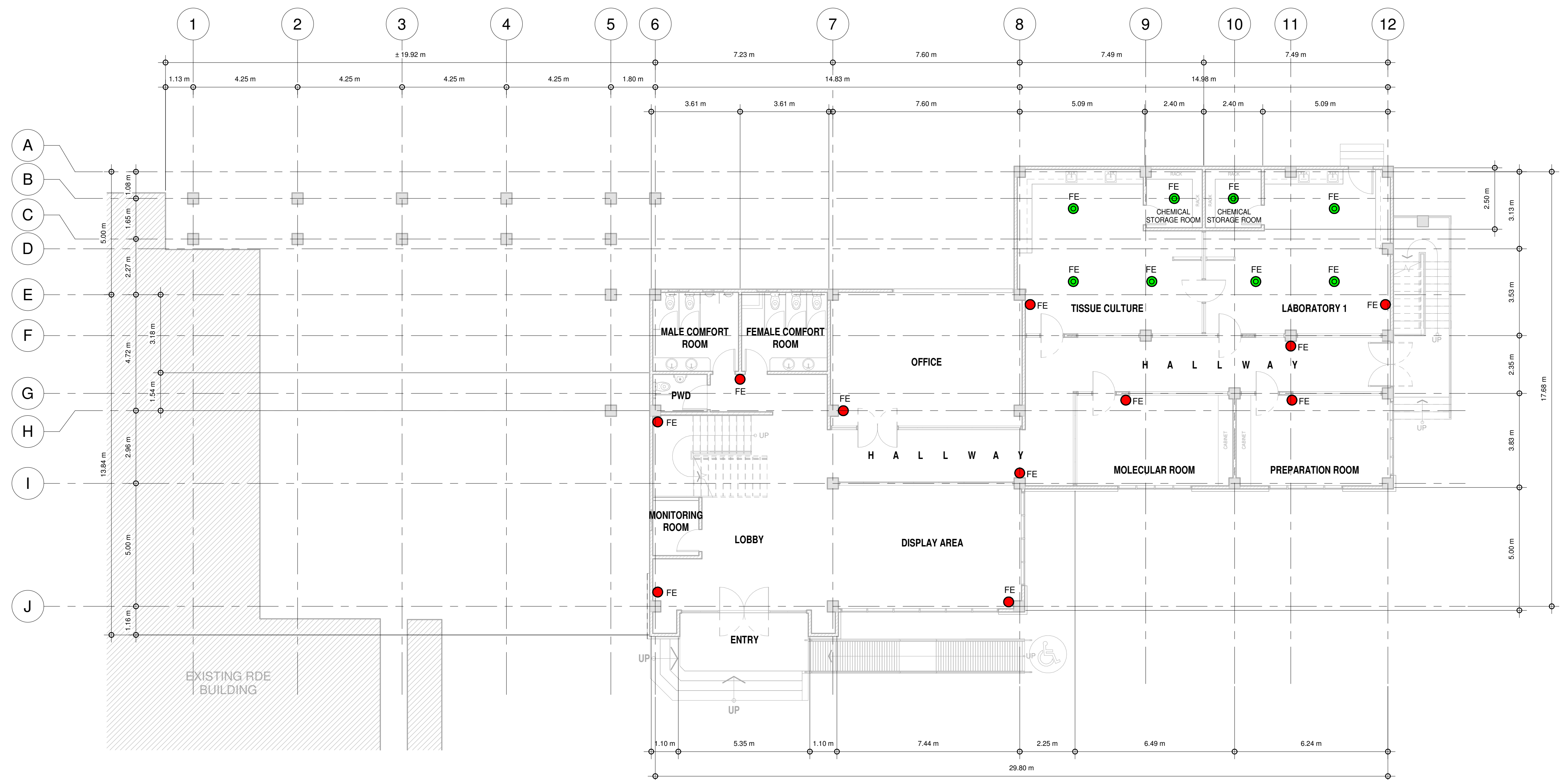
1 GROUND FLOOR FIRE EXTINGUISHER LAYOUT PLAN 1 : 100 meters
